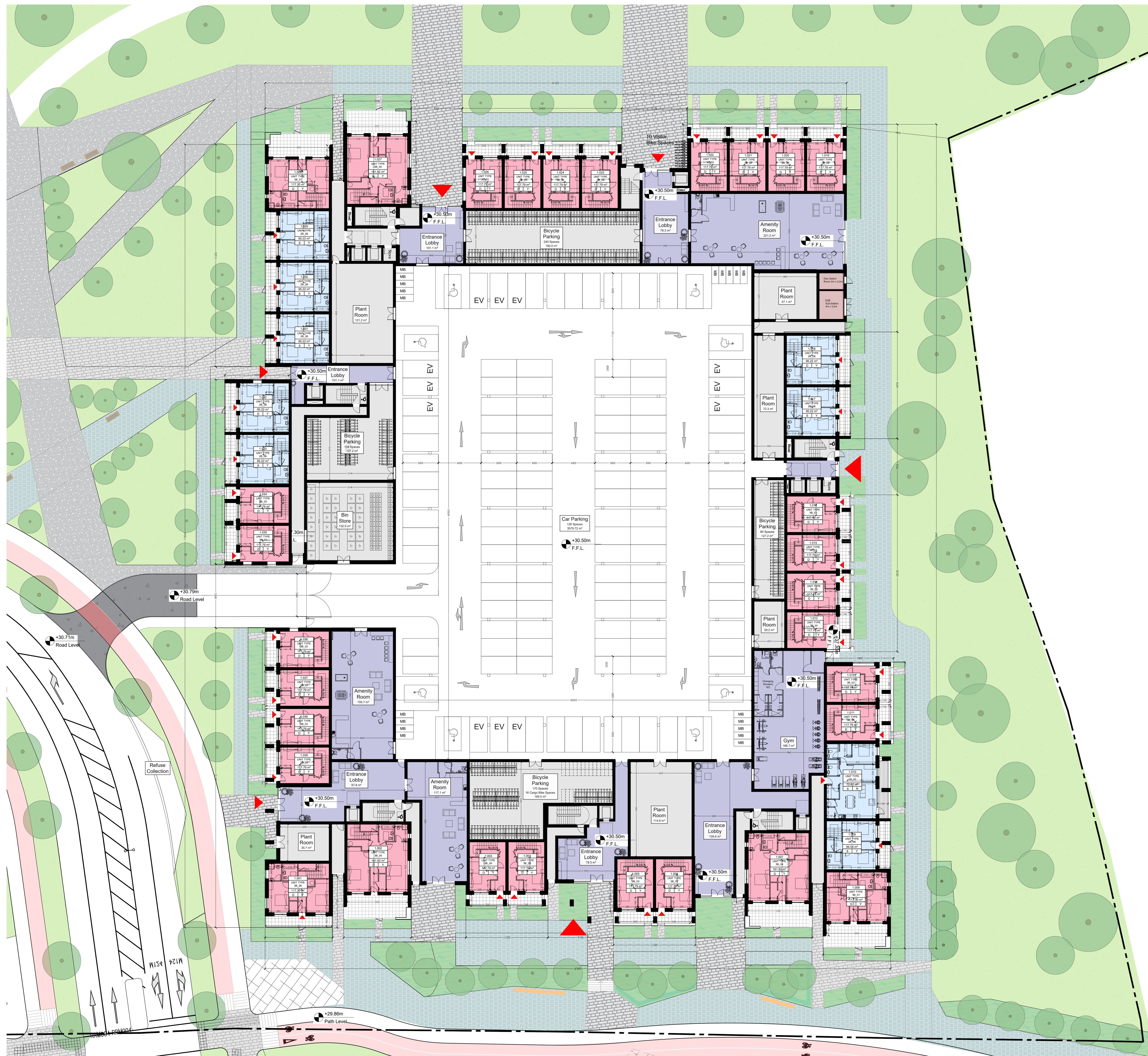
Ground Floor Plan - Block 1 Scale 1:200 @A0
